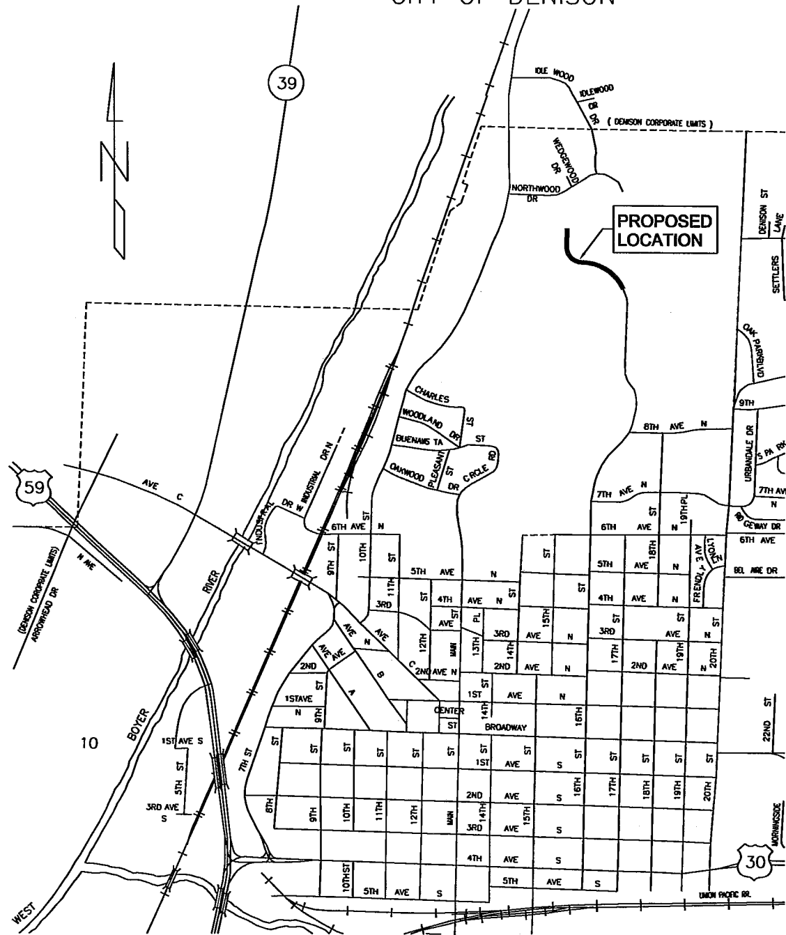
0' 800' 1600' 2400' LOCATION MAP
